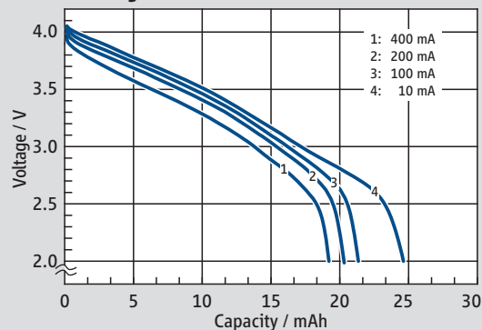
Discharge Curve at 25 °C
