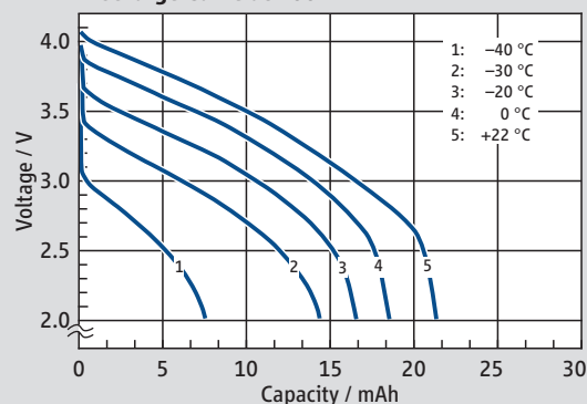
Discharge Curve at 100 mA
